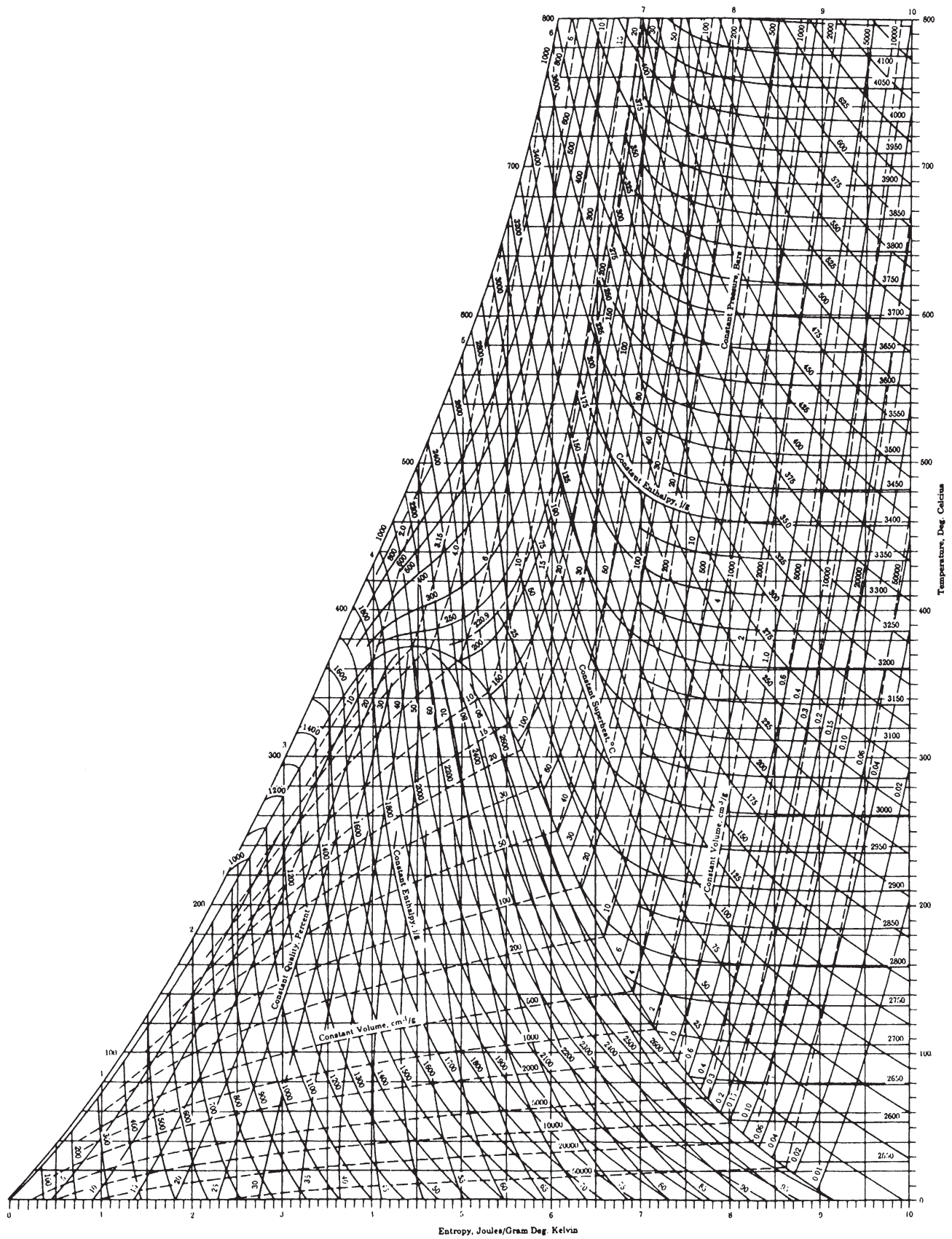
Figura E.1 Diagrama temperatura-entropia da água. Keenan, Keyes, Hill e Moore. Steam Tables (International Edition - Metric Units). Copyright ©1969, John Wiley & Sons, Inc.
